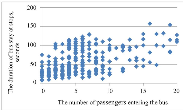
Fig. 3. The results of field studies of the duration of bus stay at the stop depending on the number of passengers entering the bus
